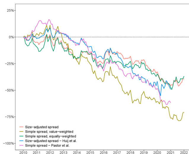
Fig. 2. Brown vs. green performance in the U.S., total emissions. Cumulative log returns for different brown-minus-green spread portfolios, based on the level of CO 2 emissions: a size-adjusted spread, a simple value-weighted quintile return spread, and a simple equal-weighted quintile return spread. Also shown are cumulative returns for the size-adjusted spread of Huij et al. (2021) , based on estimated emissions, and the simple spread of Pastor et al. (2022) , based on E-scores. Sample period: January 2010 to December 2021.
