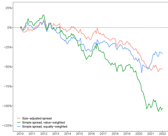
Fig. 3. Brown vs. green performance in the U.S., emission intensity. Cumulative log returns for different brown-minus-green spread portfolios, based on CO 2 emissions scaled by total scales: a size-adjusted spread, a simple value-weighted quintile return spread, and a simple equal-weighted quintile return spread. Sample period: January 2010 to December 2021.
