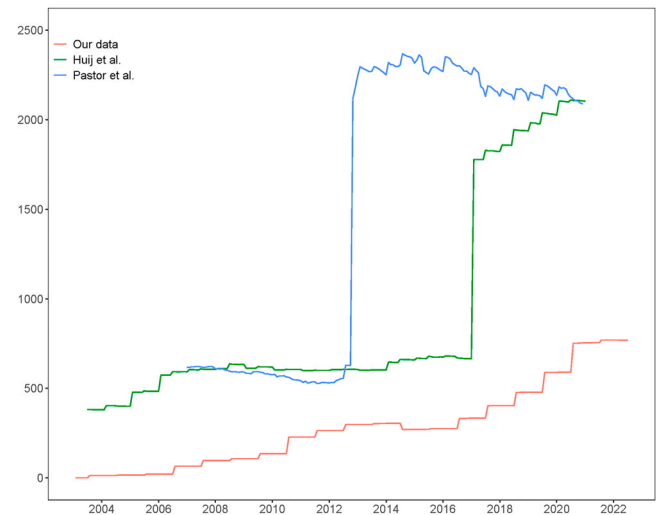
Fig. 1. Number of firms. Monthly number of firms in three data samples: our own data, which includes firms with reported emissions data from Refinitiv (using an 18-month publication lag), the data used by Huij et al. (2021), which includes firms with reported and estimated emissions data from Trucost, and the data used by Pastor et al. (2022), which includes firms with E-scores from MSCI.
