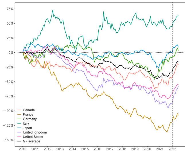
Fig. 4. Brown vs. green performance in the G7 countries, total emissions. Cumulative log returns for value-weighted, simple brown-minus-green spreads, based on emission levels, for all G7 countries as well as the average across these countries. Sample period: January 2010 to June 2022. Vertical dashed line marks the beginning of 2022, after the end of our baseline sample period.
