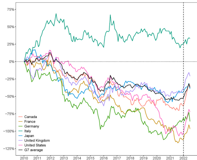
Fig. 5. Brown vs. green performance in the G7 countries, emission intensity. Cumulative log returns for value-weighted, simple brown-minus-green spreads, based on emission intensities, for all G7 countries as well as the average across these countries. Sample period: January 2010 to June 2022. Vertical dashed line marks the beginning of 2022, after the end of our baseline sample period.
